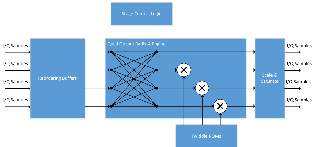
Figure 6: Radix-4 Stage Block Diagram
