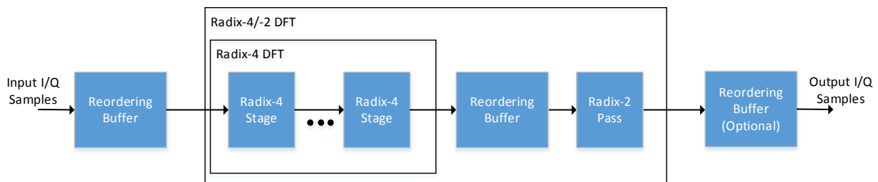
Figure 5 : Top Level Radix-4/-2 FFT Block Diagram
