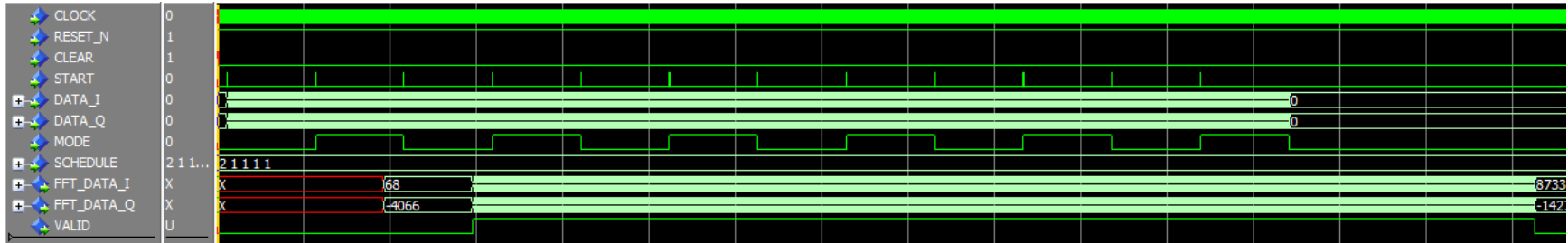
Figure 2: Overall Timing Diagram
