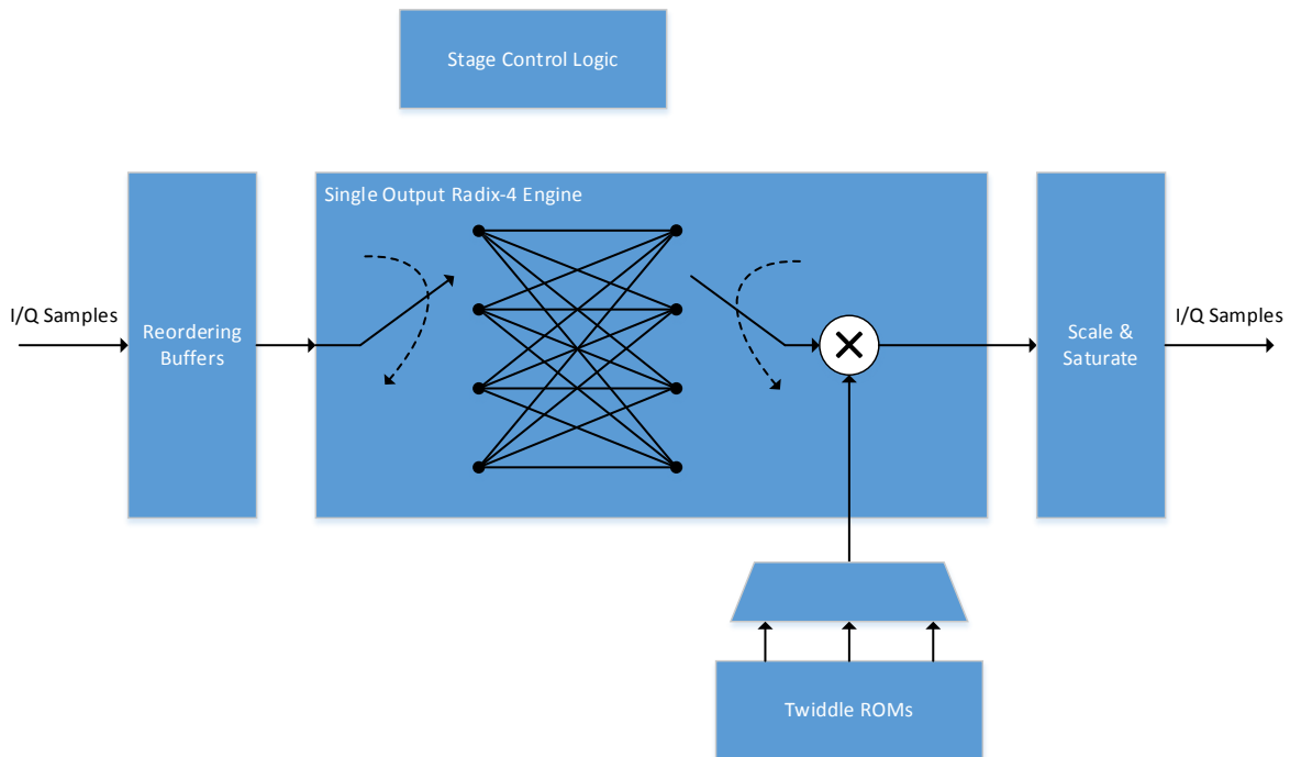
Figure 6: Radix-4 Stage Block Diagram
